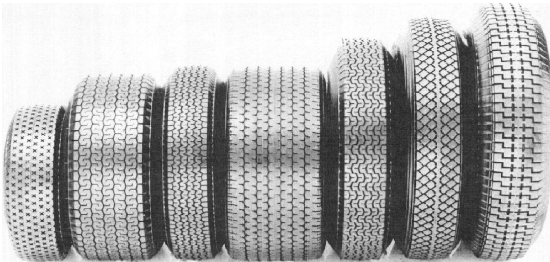
Dunlop Vintage Tread Patterns CR-70 CR-65 CR-48 CR-82 R-5 R-1 5-STUD
